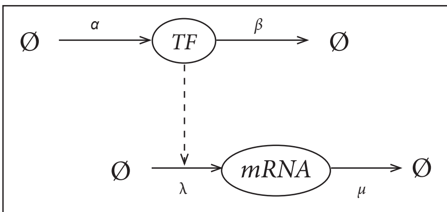
Figure 1. A graphical model of a regulated synthesis reaction
