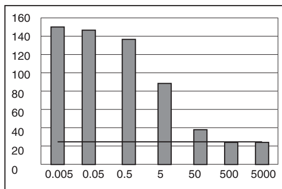
Figure 3. simulated variance of the mRNA steady-state population. The straight line is used as a control of simulation accuracy, and provides the average steady-state number of mRNA molecules
