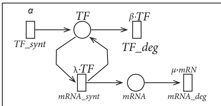
Figure 2. An SPN model for the gene expressions reactions
