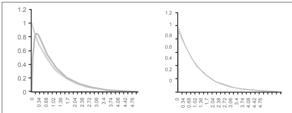
Figure 3. Comparison of occurrence time probability distributions. Left side: elementary reaction (blue-line) and two steps reaction (red line) when step 1, A+B \rightarrow Y is 10 times faster than step 2, Y \rightarrow C . Right side: elementary reaction (blue-line) and two steps reaction (red line) when step 1, A+B \rightarrow Y is 100 times faster than step 2, Y \rightarrow C .
