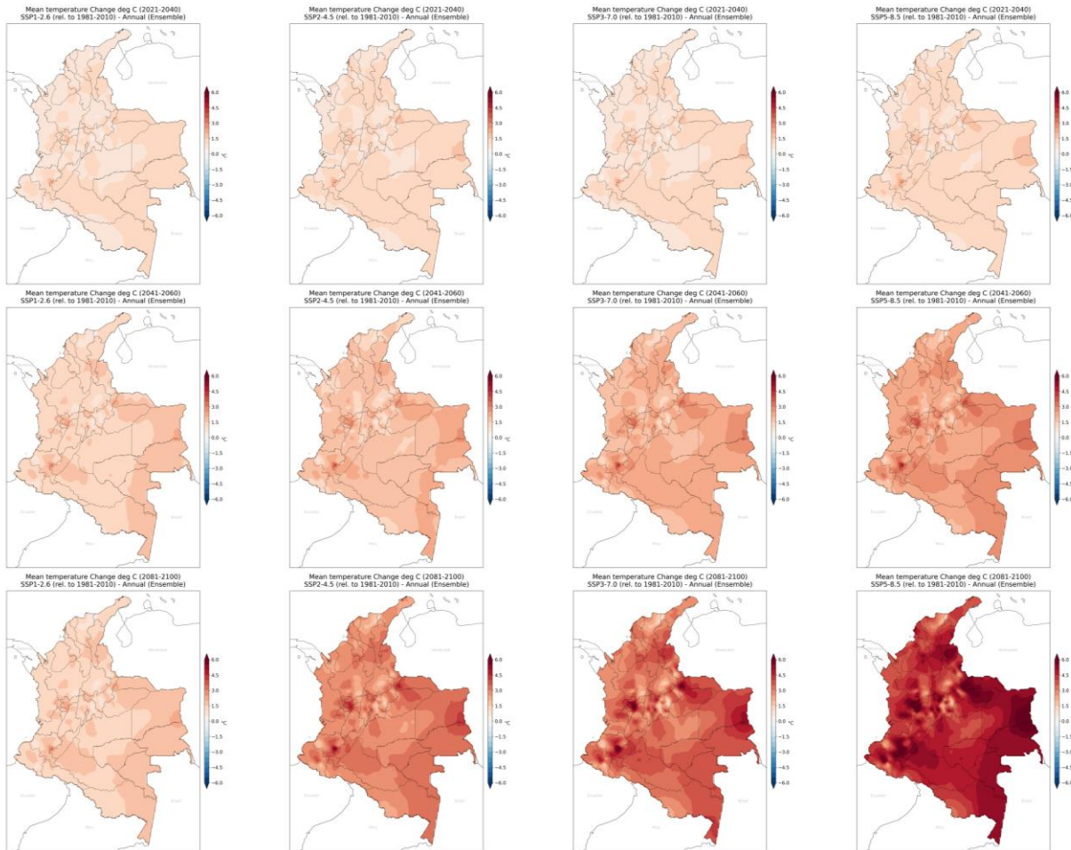
Figure 3. Estimated mean temperature change ( ^{\circ}\text{C} ) for scenarios SSP1-2.6, SSP2-4.5, SSP3-7.0, and SSP5-8.5 (from left to right) for the periods 2021-2040 (top), 2041-2060 (middle), and 2081-2100 (bottom)
